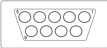
Figure 2: DB9 connector pin arrangement
