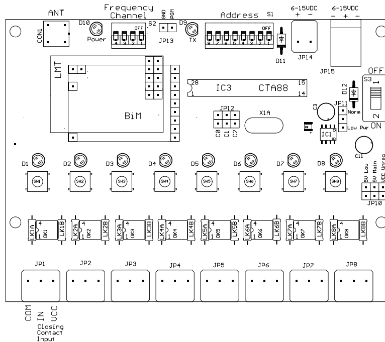
Figure 3: CTA88 TX demo board PCB (top view)
