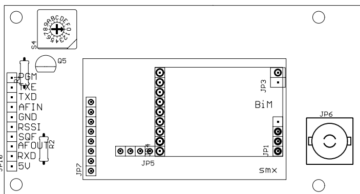
Figure 4: BiM / SMX series carrier board
