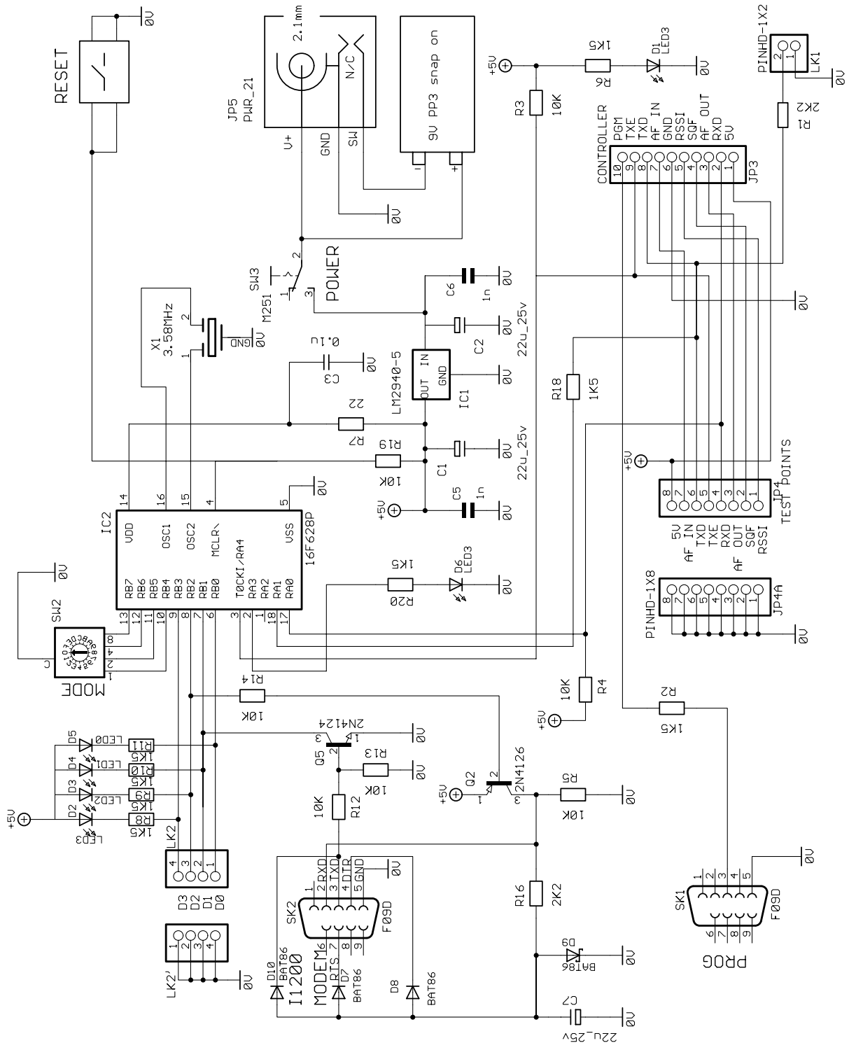
Figure 10: Schematics of main controller board
