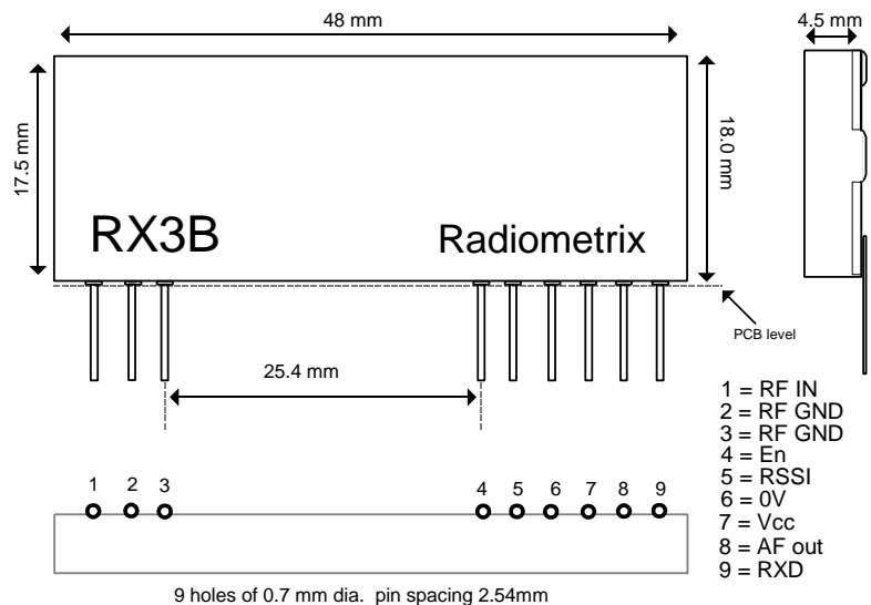
Fig.4: RX3B physical dimensions
