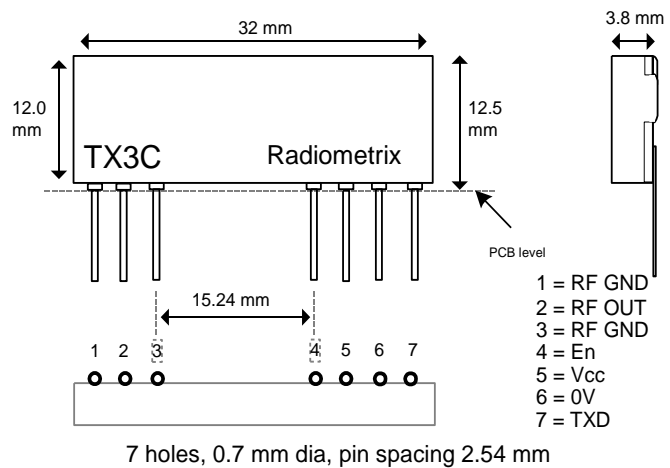
Fig2: TX3ACphysical dimensions
