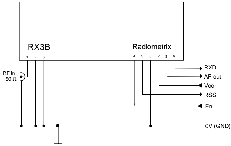
Fig.6: RX3B test circuit
