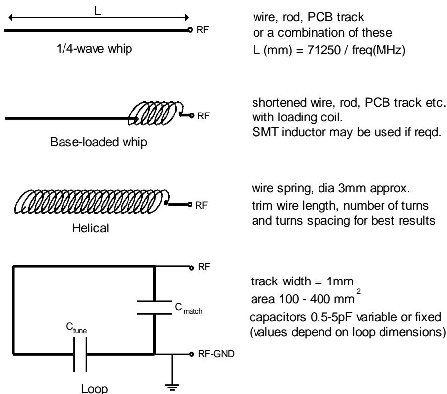
Fig.8: Integral antenna configurations
