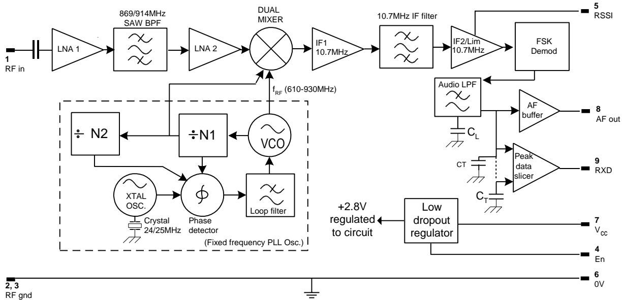
Fig.3: RX3B block diagram
