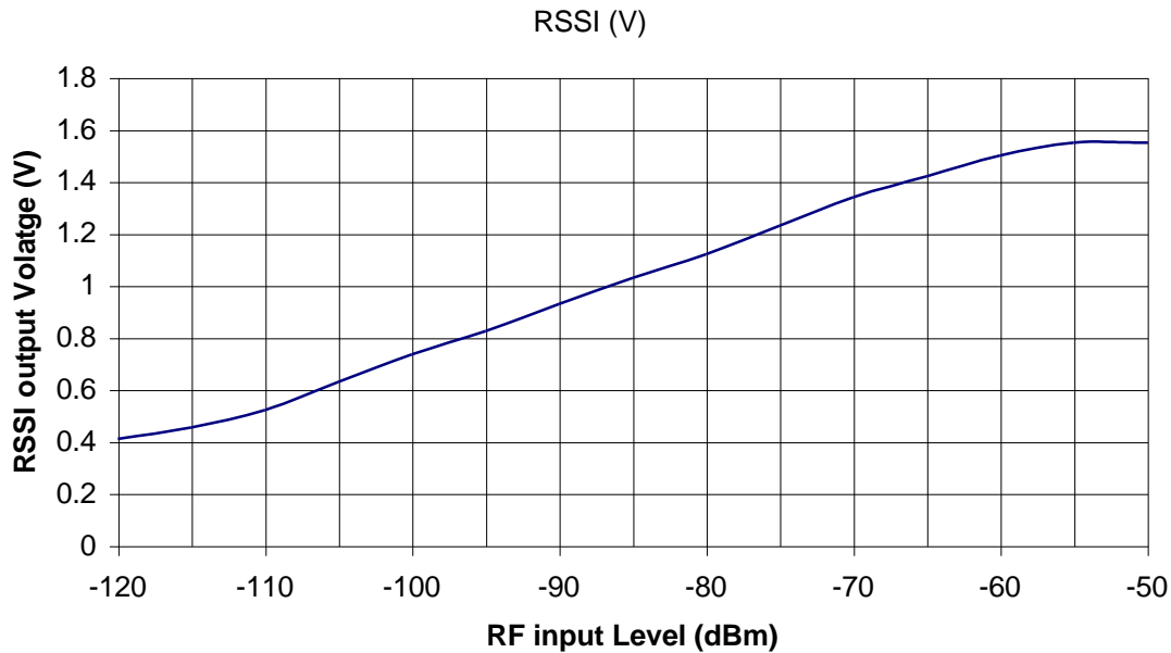
Fig.7: RX3C RSSI response curve
