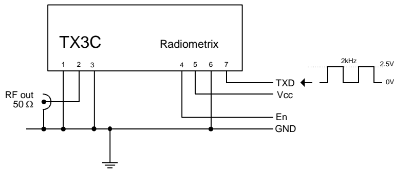
Fig.5: TX3C test circuit
