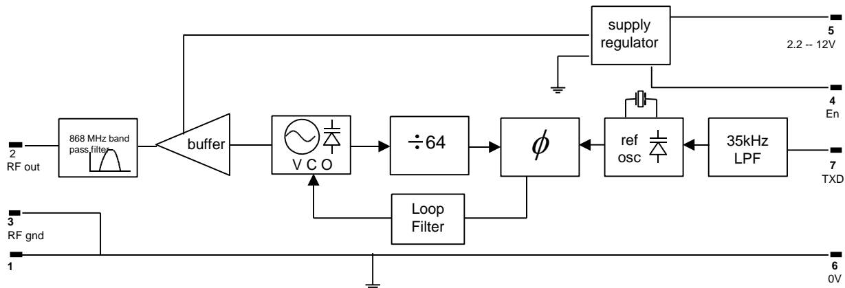
Fig 1 :TX3C block diagram
