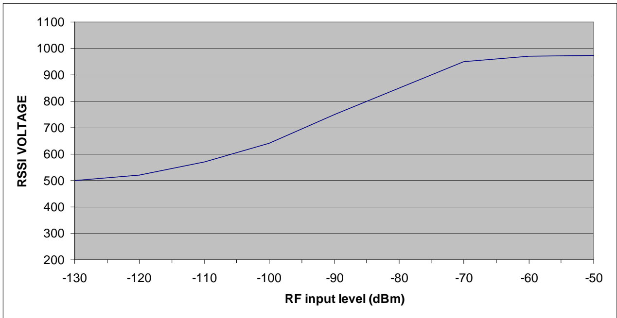
Figure 3: Typical RSSI
