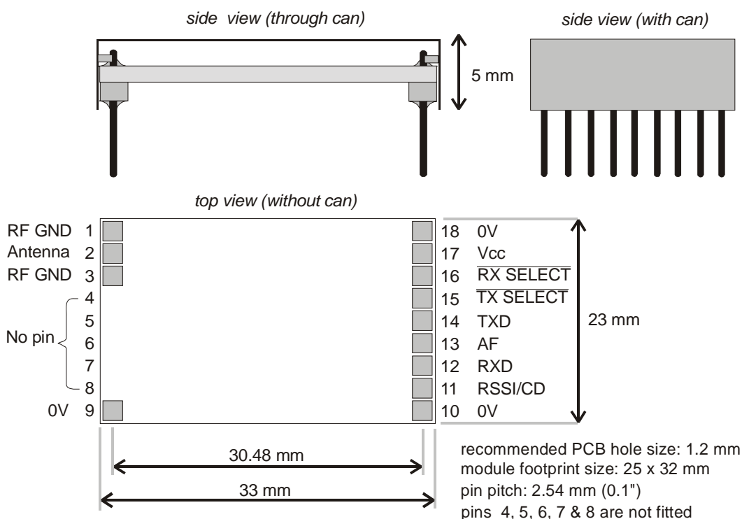
Fig. 2: Physical dimensions
